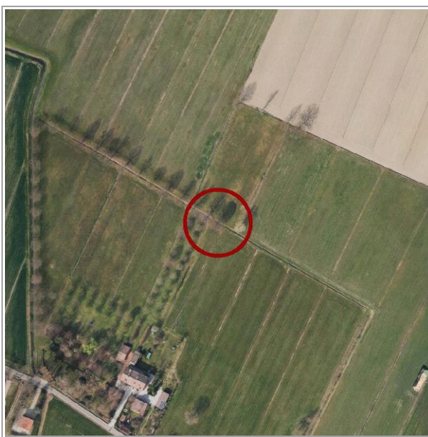
Ortofoto 2019, C.G.R.s.p.a. Parma - scala 1:5000
